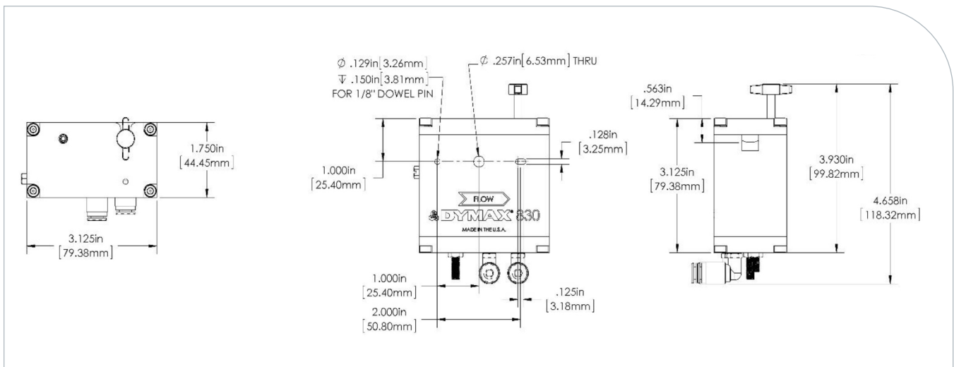
Figure 1. Model 830 Dimensions
