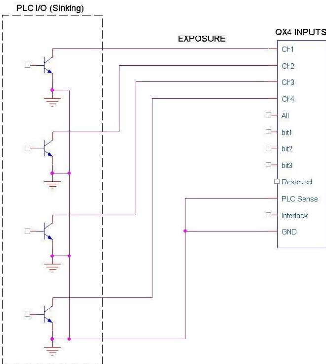
Figure 33. Connection Diagram
