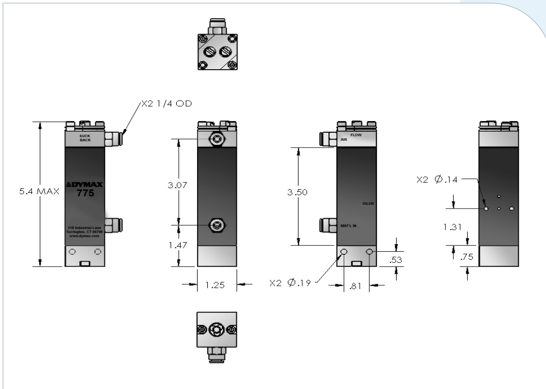
Figure 1. Model 775 Dimensions
