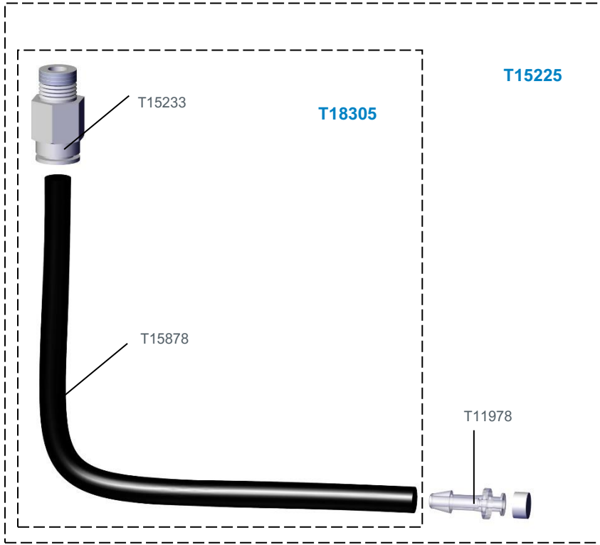
Figure 14. Tubing Assembly
