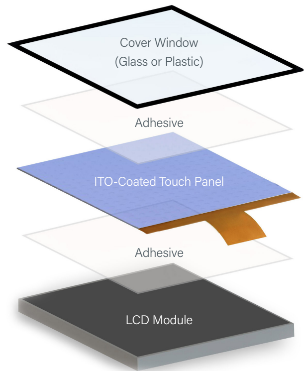
Typical Display Construction
